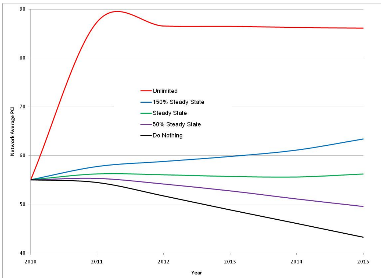
Figure 9 – Network Annual PCI Analysis Results
