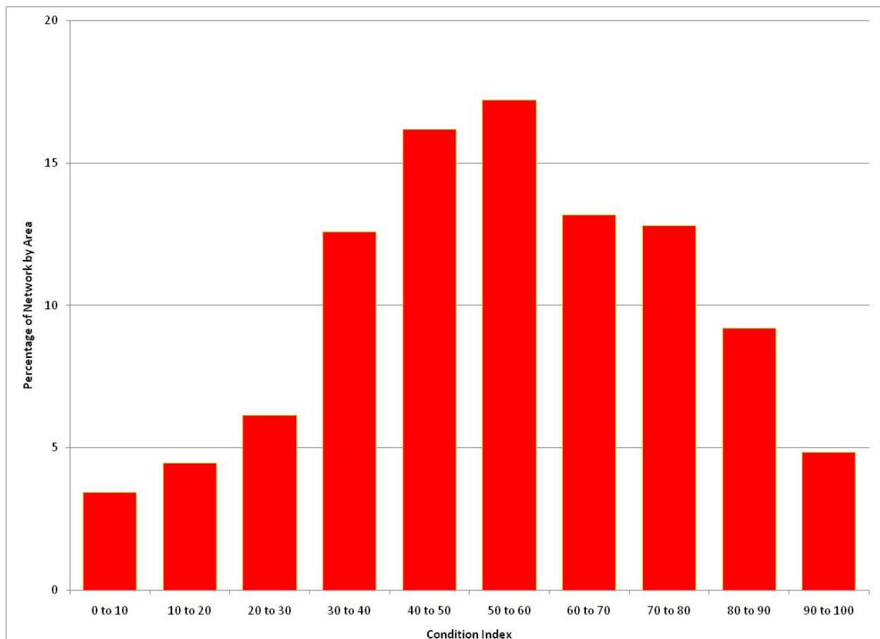
Figure 5 –Roadway Network Present Status
