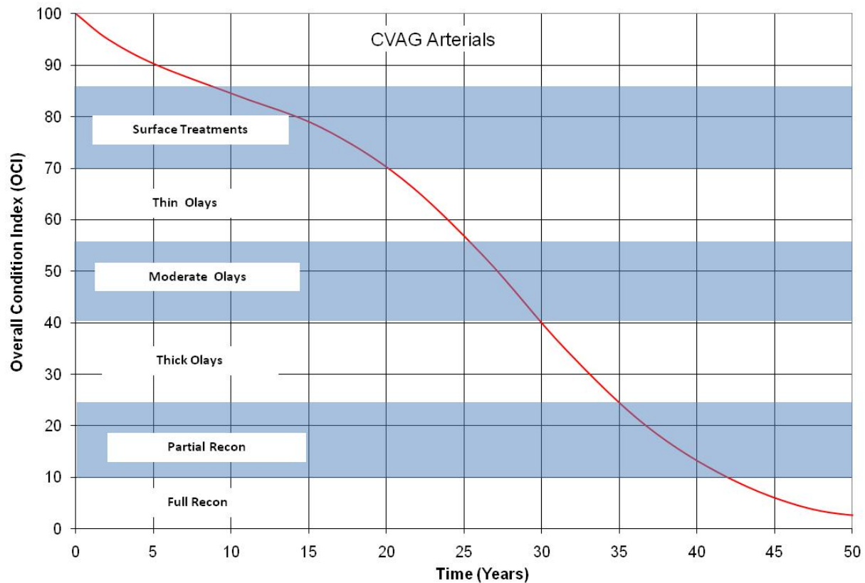
Figure 7 - CVAG Performance Curves
