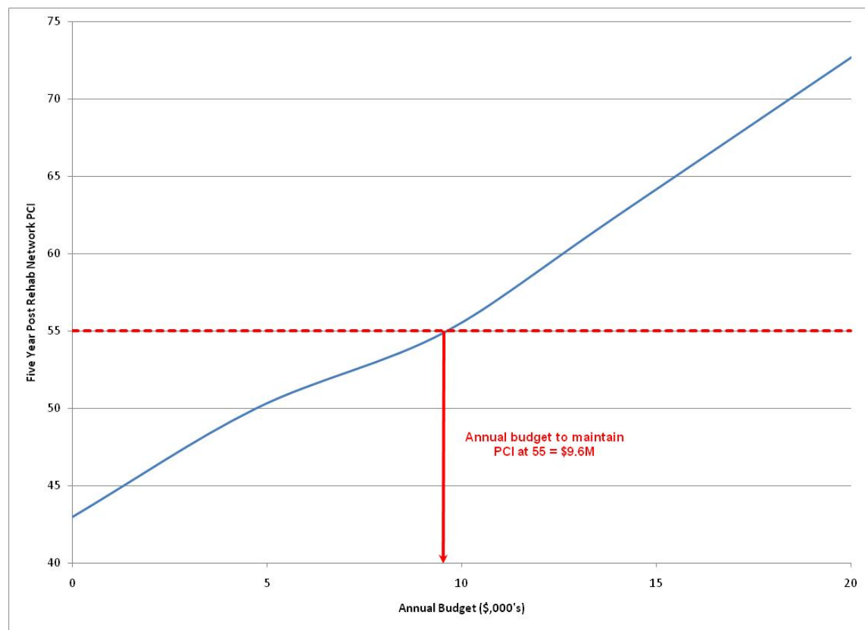
Figure 8 –5 Year Network PCI Analysis Results
